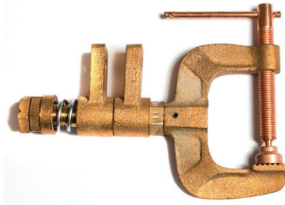
▶ ECR1000-2 Rotary Earth Clamp 1000 Amp
