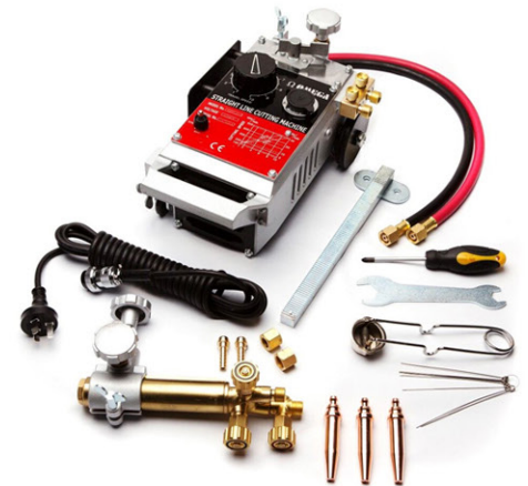
▶ BBSLC-1 No Track - Straight line cutter with/out 1.8m track
